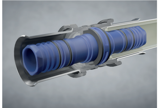
Fig.12: EASIFIT pipe insertion without calibration.
