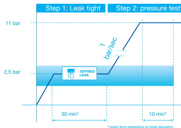
Fig. 32: Pressure test protocol when testing with water.
