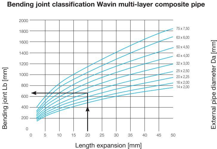
Fig. 38: Bending joint classification of Wavin multi-layer composite pipes.
