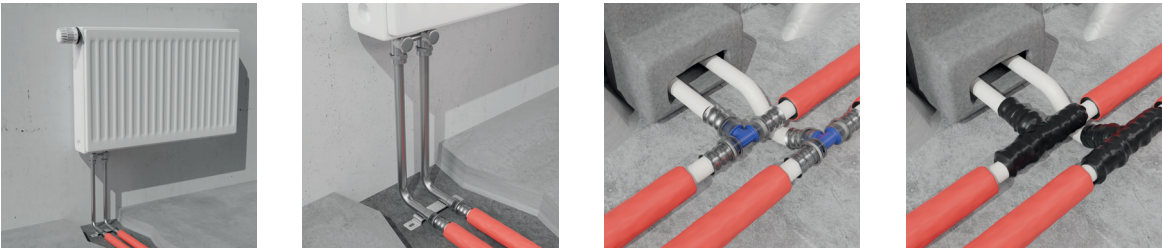
Fig. 49: Radiator installation examples with angle connection pipes.
