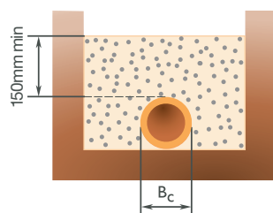
Class D Bedding Factor 1.1
