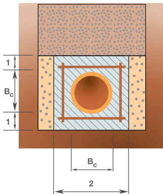
c. Reinforced concrete surround. Bedding factor 4.8 (4 × 1% steel). Reference: TRRL Simplified tables [2]
