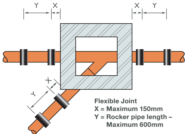
Fig. 9 – Diagrammatic sections showing pipes passing through walls
