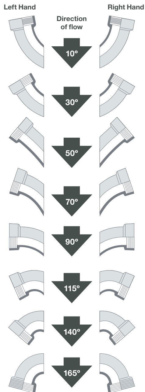
Fig. 38 – Branch channel bend selector (for half section and \frac{3}{4} section)
