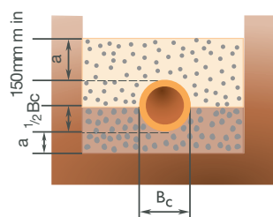
Class B Bedding Factor 2.5
