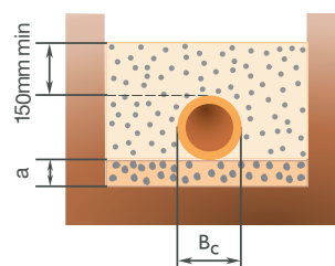
Class F Bedding Factor 1.9
