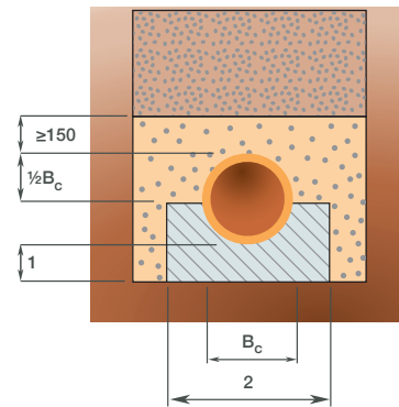
d. Unreinforced concrete bed. Bedding factor 2.6
